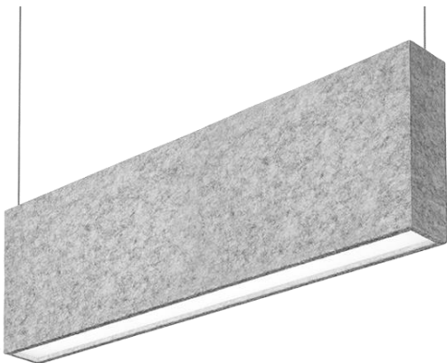
FOCAL POINT: ACOUSTICAL DIRECT/INDIRECT SUSPENDED LIGHT
